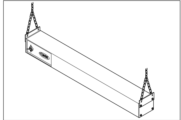
Figure 3. Standard Bracket Mounting with Chains
