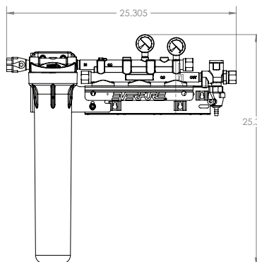
Coldrink/Insurice Triple Manifold with 20" Prefilter: EV9293-23
