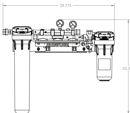
High Flow Triple Manifold with CSR 20" Prefilter: EV9294-23
