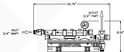
QC71 Triple Head: EV9272-23
